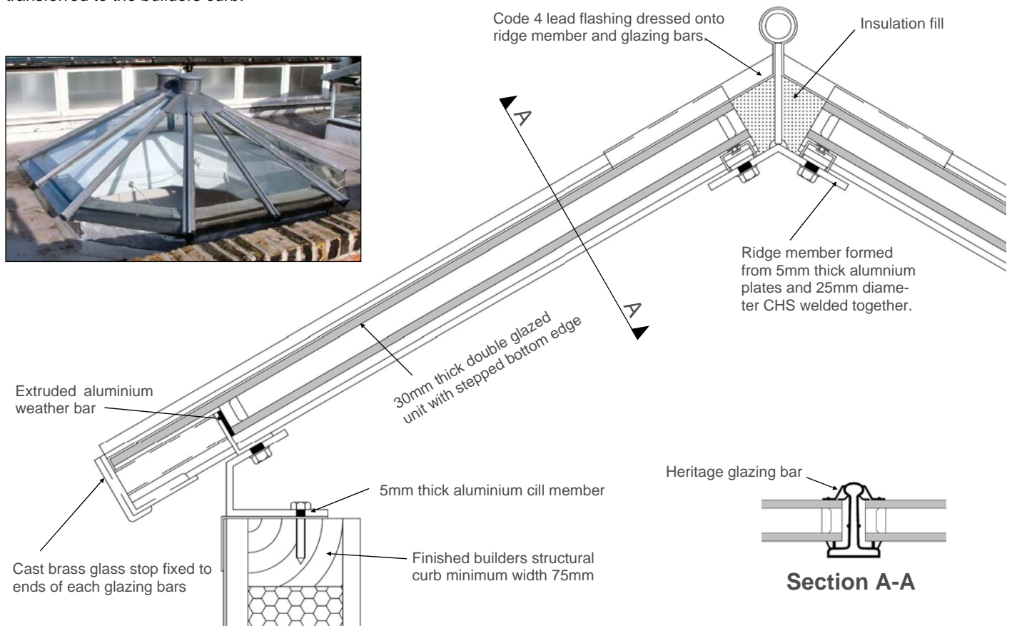
Section through Heritage Hipped Skylight Scale 1:4
