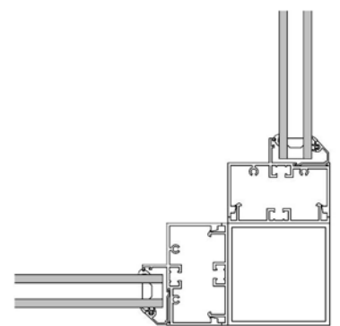
Section at corner post
